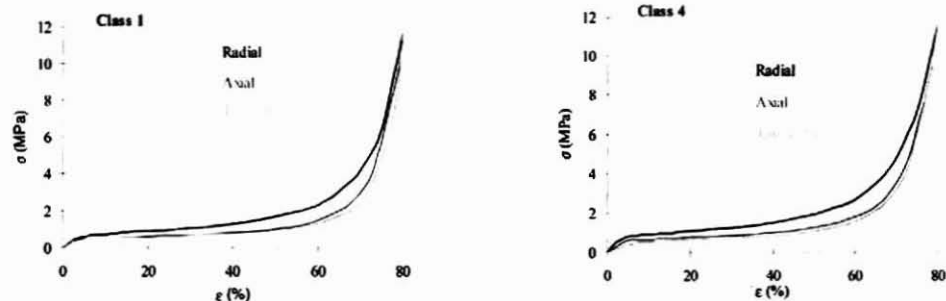
Figure N° 1 STRESS-STRAIN CURVES FOR THE COMPRESSION OF CORK SPECIMENS OBTAINED FROM CORK PLANKS OF CLASS 1 AND CLASS 4 IN THE THREE DIRECTIONS (RADIAL, AXIAL AND TANGENTIAL).
